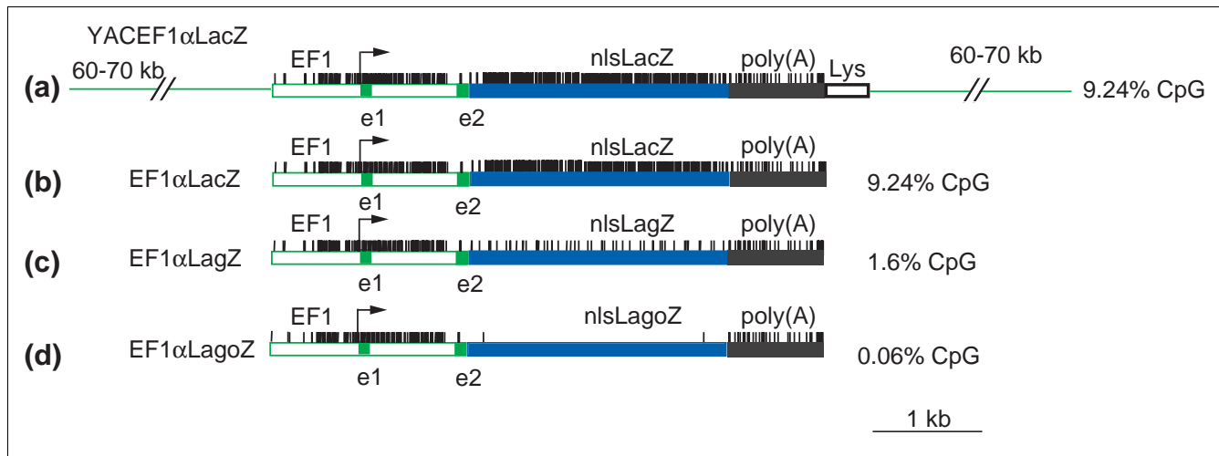
Figure 1 EF1 \alpha LacZ reporter genes with different CpG content. All four constructs share the same promoter region (EF1) from the human EF1 \alpha (translation elongation factor 1, \alpha subunit) gene including the exon 1 (e1) and a part of exon 2 (e2), a polyadenylation sign (poly(A)) from Moloney murine virus and a nuclear locating signal (nls) from the large T antigen of SV40 [32]. Both the left and right arms of the YAC (green line) are 60-70 kb long. Each vertical bar corresponds to a CpG dinucleotide. The percentage of CpGs in the reporter gene is indicated on the right.
